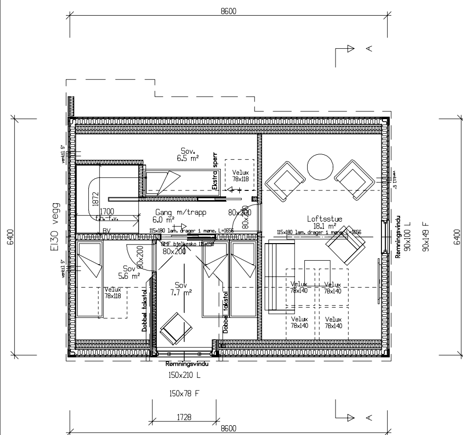
Loftsplan Bra=35,1m 2
