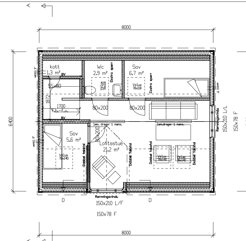
Loftsplan Bra=30,2m 2
