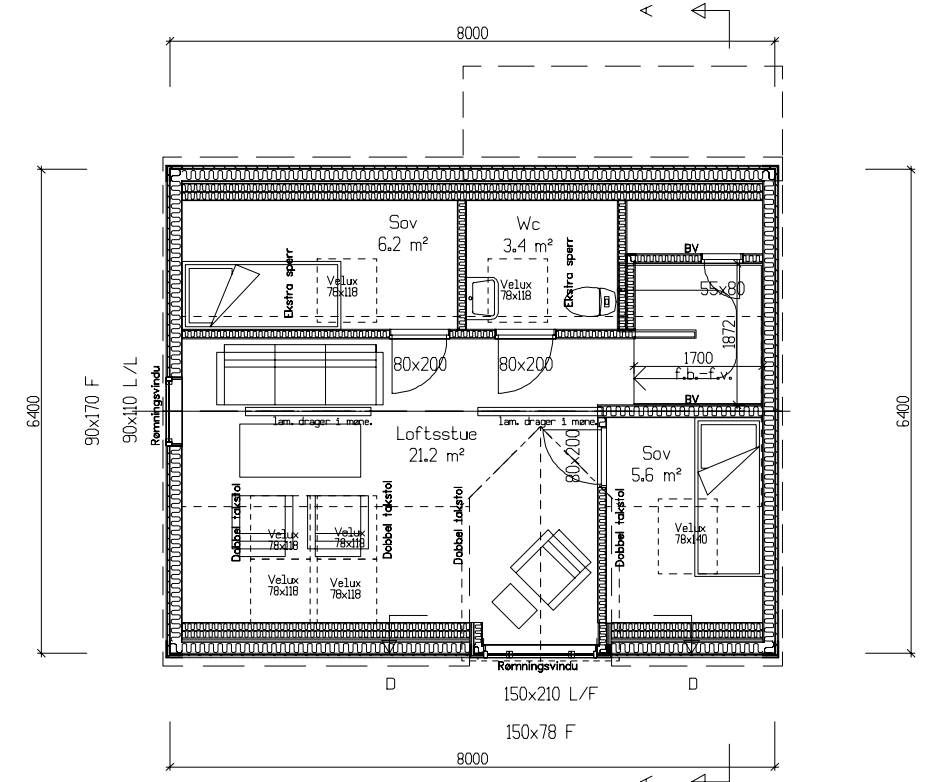
Loftsplan Bra=30,2m 2
